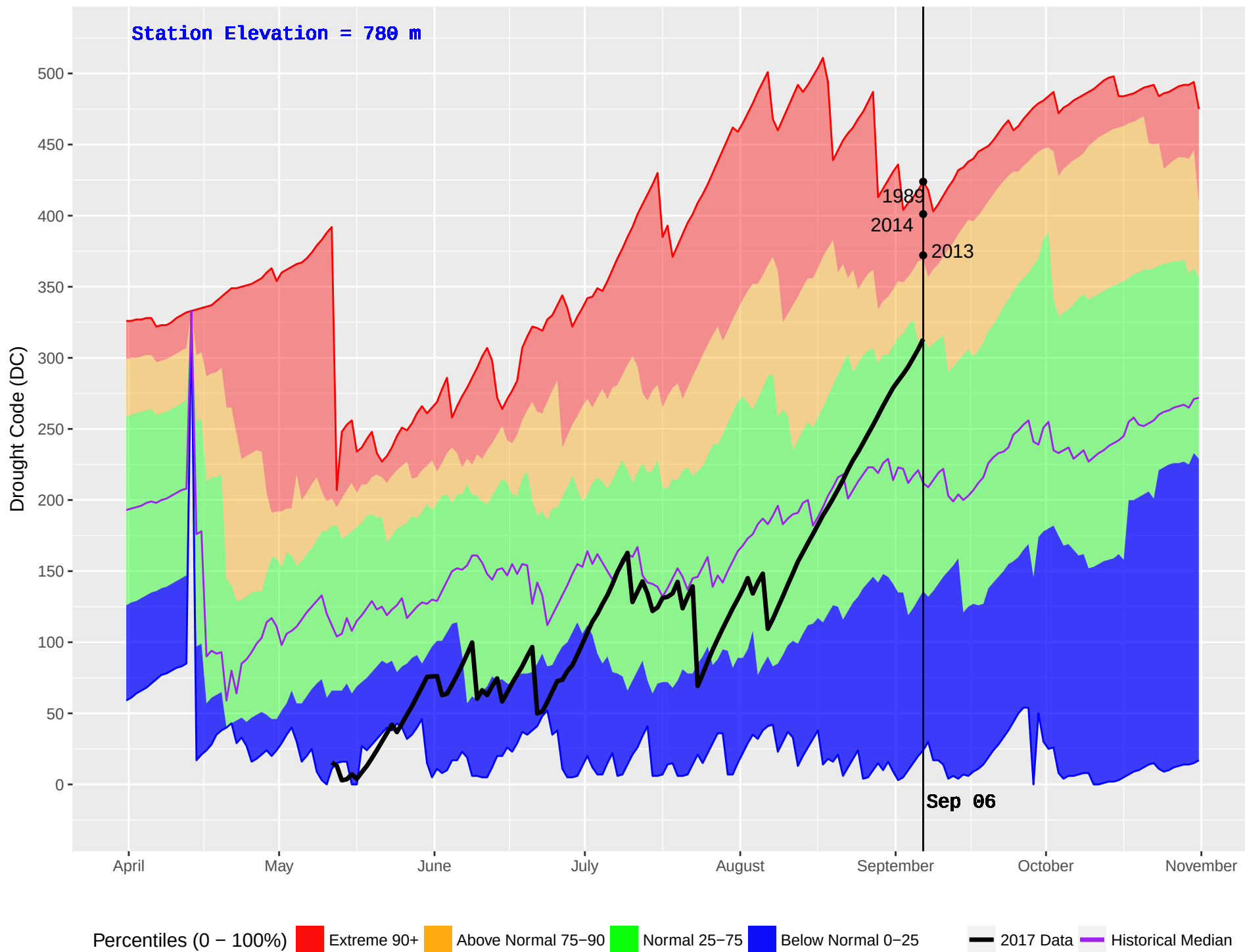
MUSKWA (131) : Historical (1983–2016) and Current (2017) Noon Drought Code (DC)
